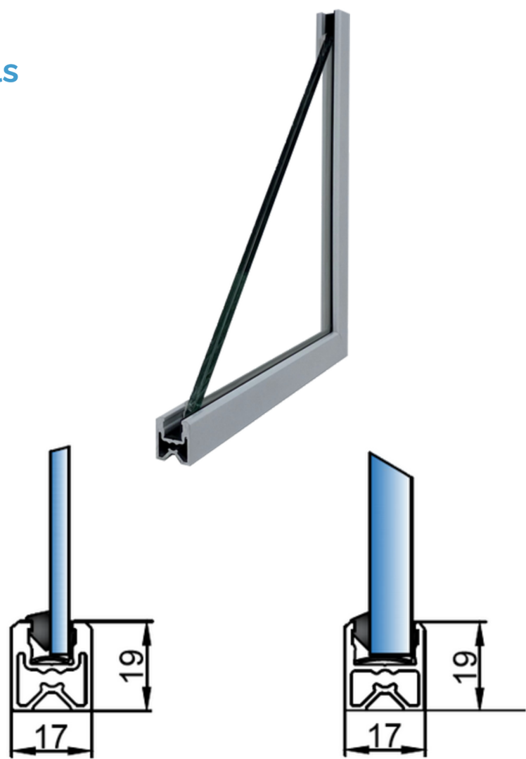
Standard Frame 4mm to 6.6mm glass sizes
