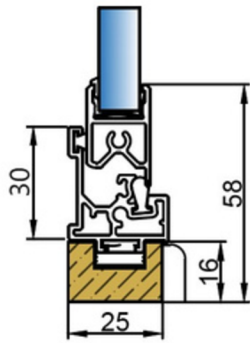
Standard Frame Ultra-Panel
