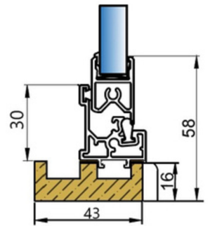
XL Frame Ultra-Panel
